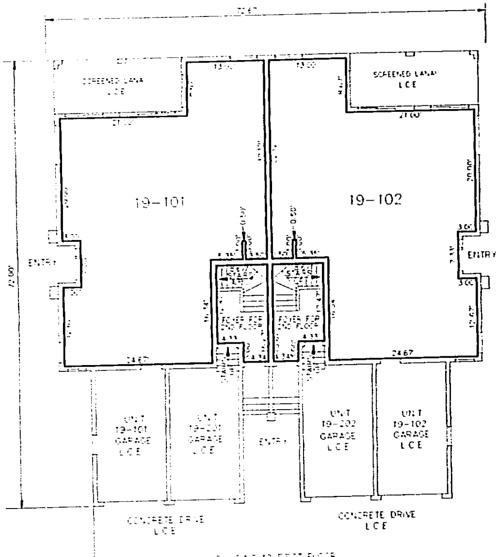
BUILDING FIRST FLOOR
